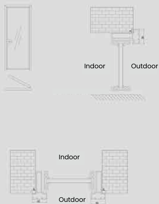
Italian-style Yunde single-package hinged door assembly diagram
