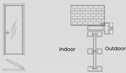
Italian-style patchwork single-pack hinged door assembly diagram
