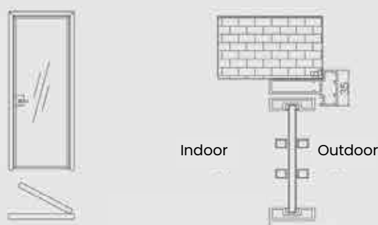
Italian-style light and shadow single-pack hinged door assembly diagram
