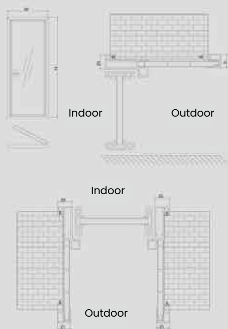
Italian-style cloud mirror double-walled hinged door assembly diagram
