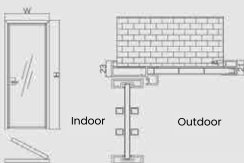
Italian-style double-sided swing door assembly diagram
