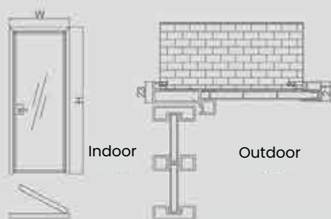
Italian-style patchwork double-sided hinged door assembly diagram
