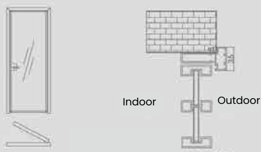
Italian-style patchwork single-pack hinged door assembly diagram
