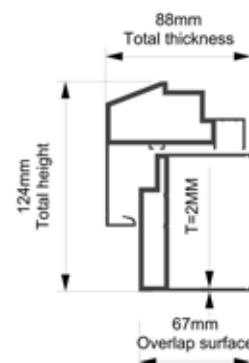
Material: 6063-T5 Aluminium profile
